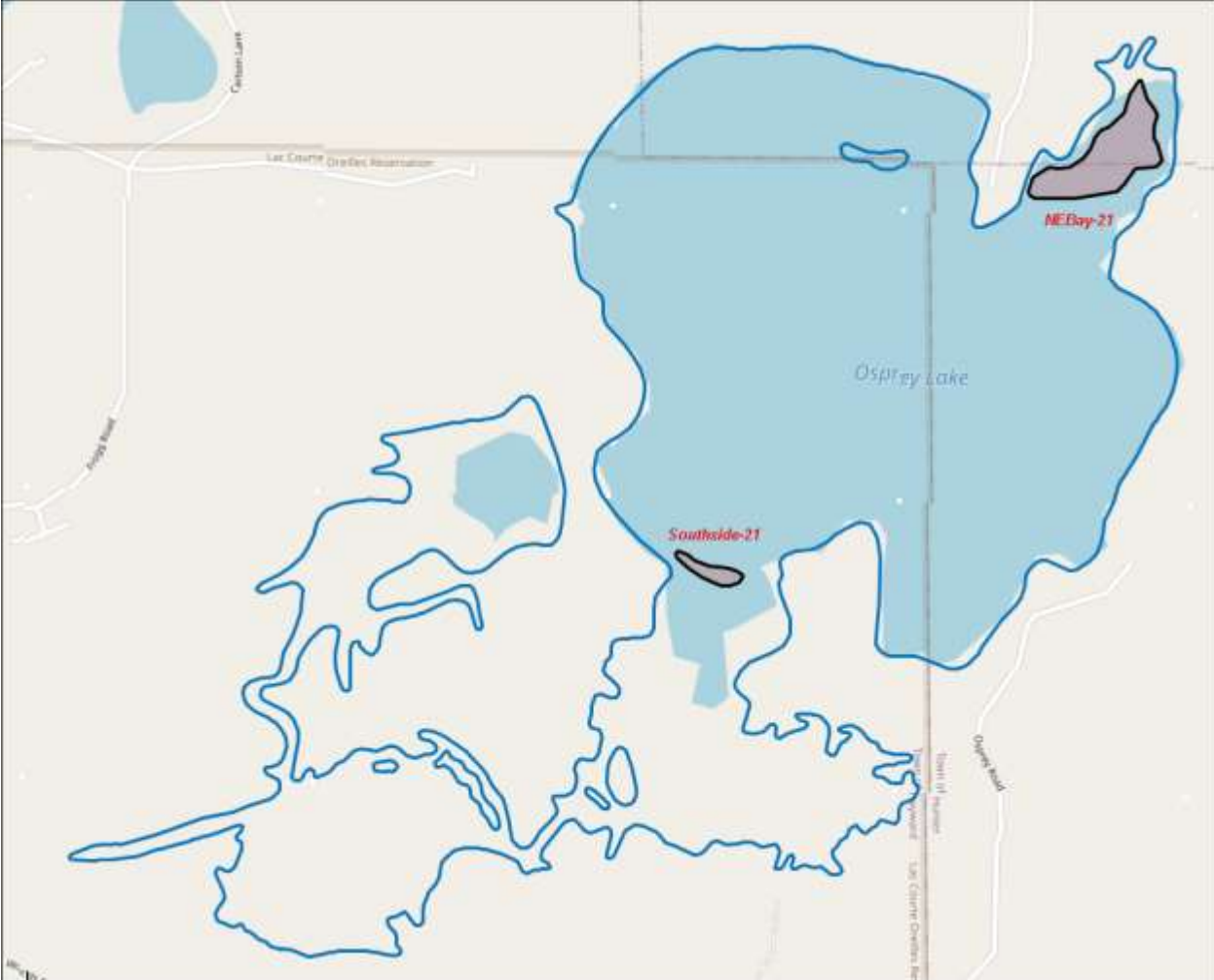
Figure 1: 2021 EWM management areas in Osprey Lake, Sawyer County
