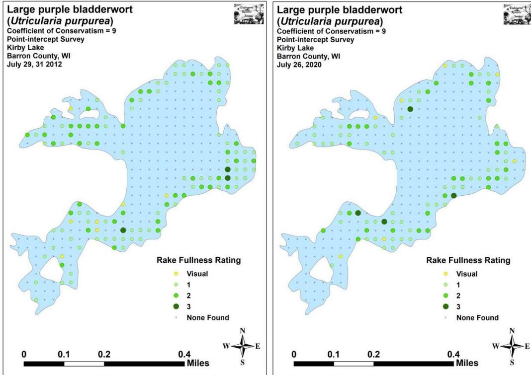
Figure 8: 2012 and 2020 Large Purple Bladderwort Density/Distribution (Berg, 2020)
